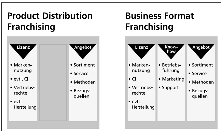
Abbildung 1: Product-Distribution-Franchising – Business-Format-Franchising
